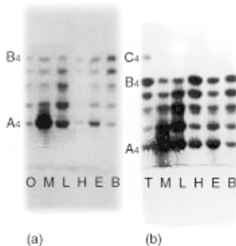
Fig. 1. Lactate dehydrogenase isozymes of Hemidactylus frenatus . A 4 predominates in skeletal muscle, B 4 in heart, and C 4 in testes. Note that the C 4 homopolymer is highly anodal and was only detected in testes. (a) Gel run using extracts of female lizard. (b) Gel run using extracts of male lizard. B, brain; E, eye; H, heart; L, liver; M, skeletal muscle; O, ovary; T, testis.
