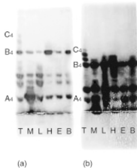
Fig. 2. Lactate dehydrogenase isozymes of (a) Eumeces elegans and (b) Mabuya longicaudata . C_4 homopolymer is highly anodal and was only detected in testes. For abbreviations see figure 1.
