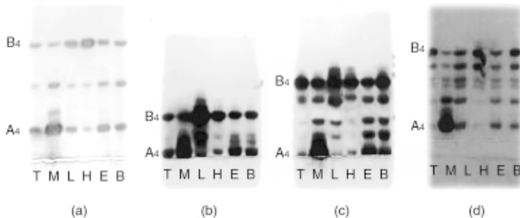
Fig. 3. Lactate dehydrogenase isozymes of (a) Takydromus formosanus , (b) Scincella formosensis , (c) Sphenomorphus indicus , and (d) Japalura mitsukurii . For abbreviations see figure 1.
