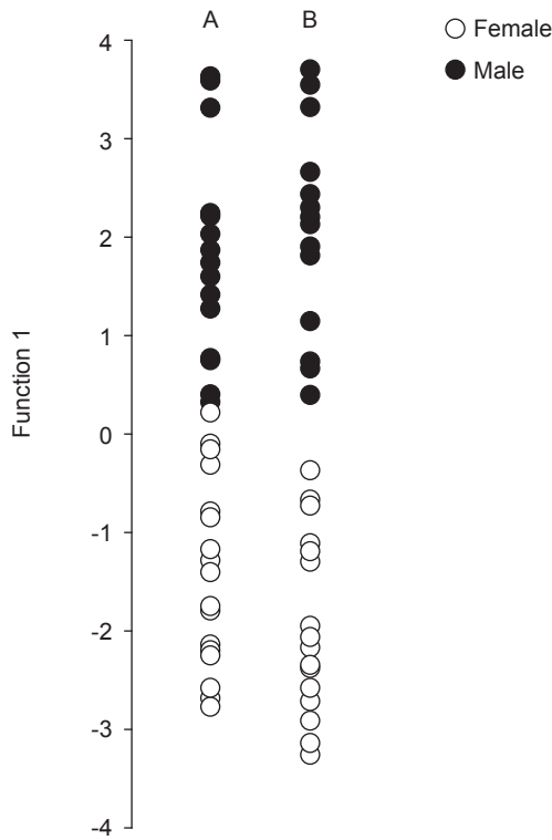
Fig. 2. Discriminant functions registered for (A) linear, angular, and area variables, and (B) shape variables of the heel pad. Solid circles are males, and open circles are females.
