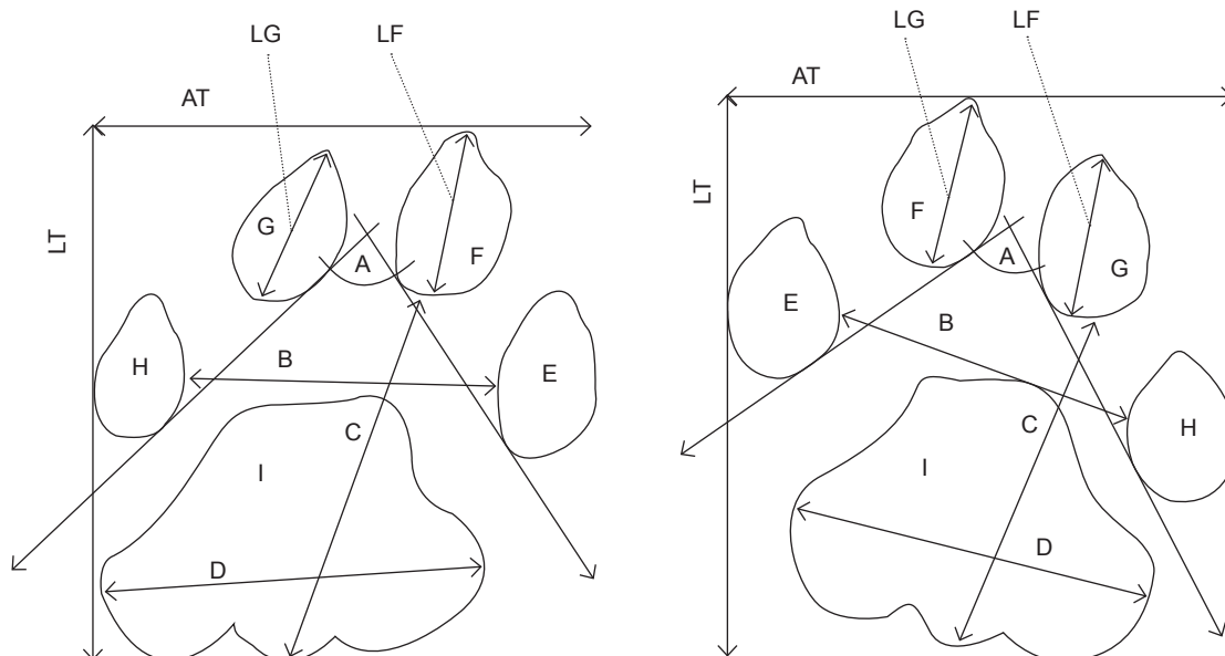
Fig. 1. Measures of left and right puma tracks. (A) Angle between inner toes; (B) outer toe spread (the line is the midpoint of each toe); (C) heel to lead toe length (line from the midpoint of the central lobe of the heel pad to the midpoint of the 3rd toe); (D) heel pad width (line of maximum width); (E) area of inner toe; (F) area of the 2nd toe; (G) area of 3rd toe; (H) area of outer toe; (I) area of heel pad. LG, length of the 3rd toe; LF, length of the 2nd toe; TL, total length; TW, total width.
