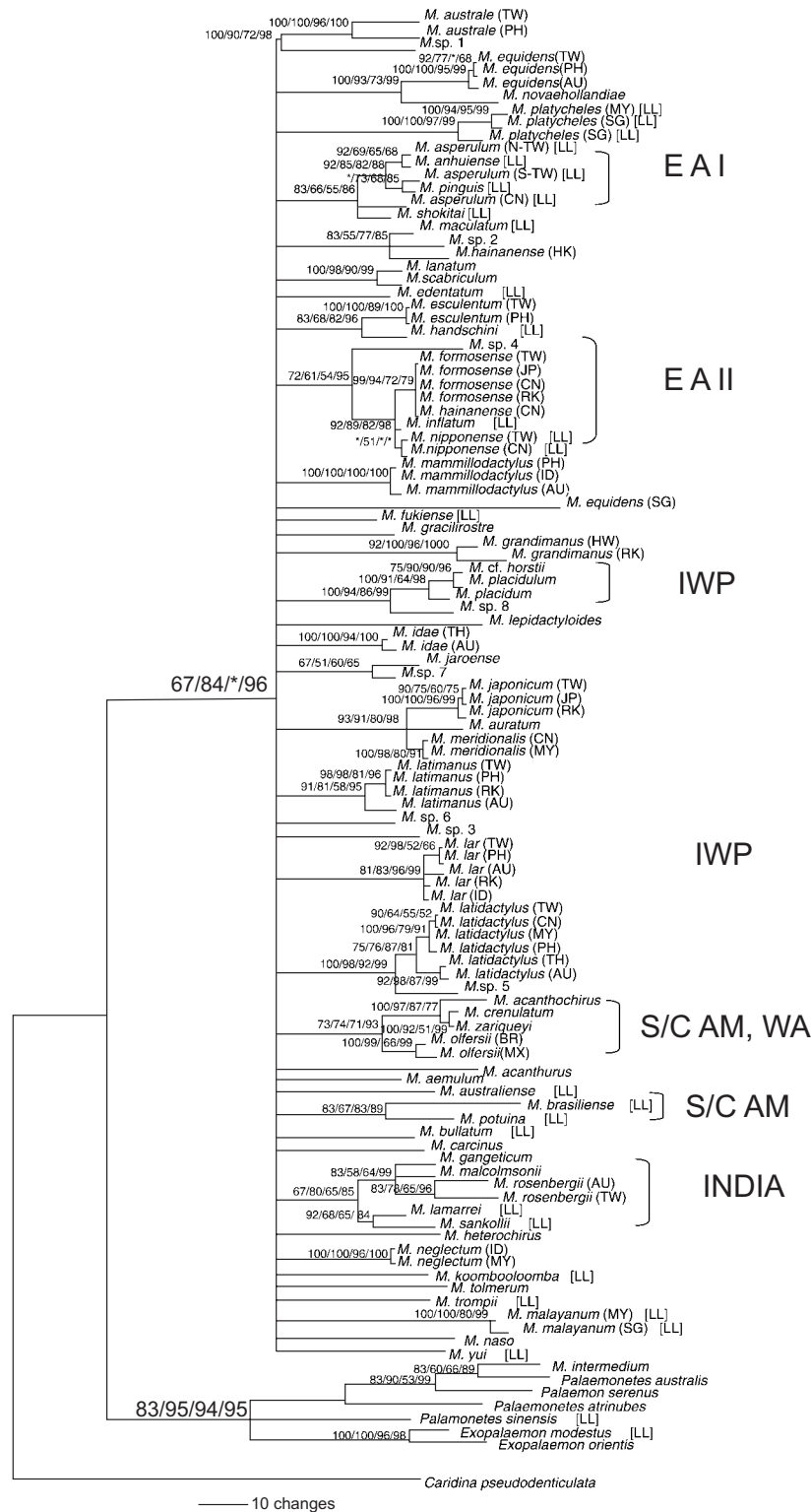
Fig. 2. Phylogenetic relationships based on large subunit (16S) sequences represented by a maximum parsimony (MP) 50% majority tree. Numbers on the branches indicate bootstrap values for the Neighbor-joining (NJ), MP, and maximum-likelihood (ML) analyses, and Bayesian analysis (BI). LL, land-locked species; EA, East Asia; IWP, Indo-West Pacific; S/C AM, South/Central America; WA, West Africa. EA I and EA II, 2 species groups found in East Asia. Abbreviations in brackets after the species names are the locality codes, which are given only when multiple samples of species were collected from different localities to assess the monophyly of the putative species. Locality codes are explained in tables 1 and 2. An asterisk (*) indicates a bootstrap value of < 50.
