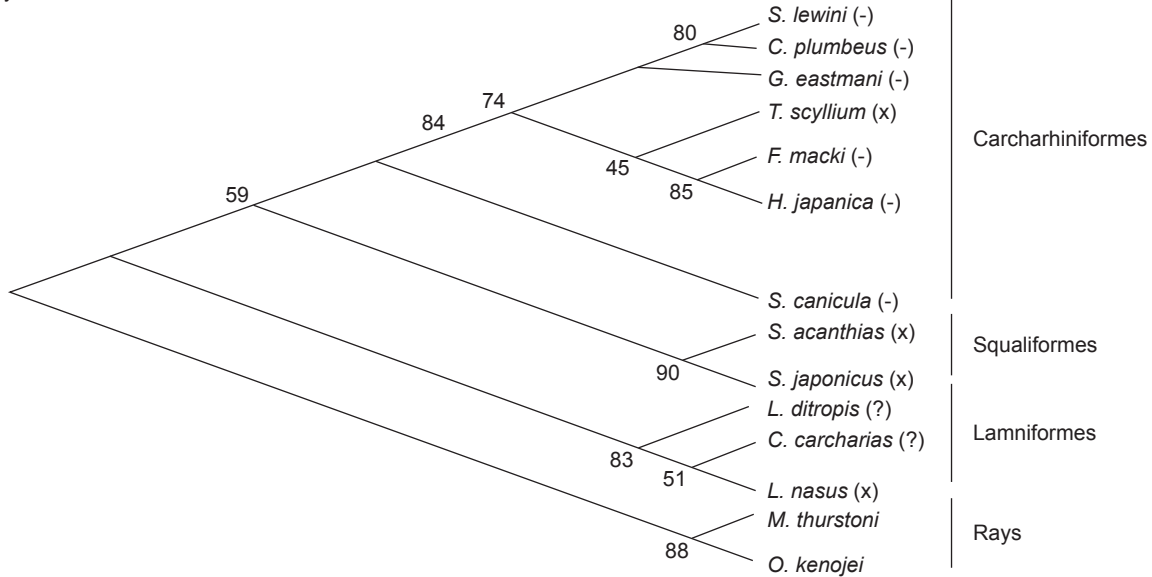
Fig. 1. Phylogenetic relationships within clades of shark orders with their family members, based on cytochrome a 3 , subunit 1 sequences (A), or cytochrome b + 16S rRNA sequences (B). The full systematic names of individual species, as indicated at the right-hand side of the branches, can be found in "MATERIALS AND METHODS", including order and family names (Table 1). A few other names of sharks, studied earlier (Schuurmans Stekhoven et al. 2001) are Lamna nasus (Lamniformes: Lamnidae), Squalus acanthias (Squaliformes: Squalidae), Scyliorhinus canicula (Carcharhiniformes: Scyliorhinidae), and Triakis scyllium (Carcharhiniformes: Triakidae). Since no cytochrome a 3 -1 data were available from L. nasus , some additional sequences of family members ( Carcharodon carcharias , Isurus paucus , I. oxyrinchus , and L. ditropis ) were used to construct the Lamniformes clades. Accession nos. are given in "Materials and methods". Sharks containing the phospholemman sequences in the 12-15 kDa region, and hence probably in their cell membrane, are indicated by the letter 'x'. Phospholemman sequences found in the 16-18 kDa region are indicated by the letter 'o', suggesting that they may occur in the cytoskeleton. The absence of phospholemman from the rectal gland is indicated by a minus sign (-). Sharks of the family Lamnidae introduced to locate their position in the phylogenetic tree, but not analysed for the presence of phospholemman, are indicated by a question mark (?). The 2 outgroup rays ( Okamejei kenojei and Mobula thurstoni ) were only used to construct the phylogenetic tree of sharks and were not analysed for the presence or absence of phospholemman in this study.
