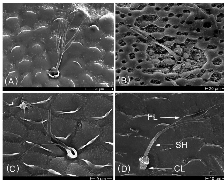
Figure 4 Scanning electron micrographs of the microtrich structures of Sphaeroma , Dynamenella , and Cymodoce species. (A) Sphaeroma khalijfarsi (with short collar and shaft, long filaments). (B) Sphaeroma walkeri (with short collar, long shaft, long filaments). (C) Dynamenella granulata (with short collar and shaft, long filaments). (D) Cymodoce sp. (with medium collar, very long shaft and filaments); CL, collar; SH, shaft; FL, filament.
