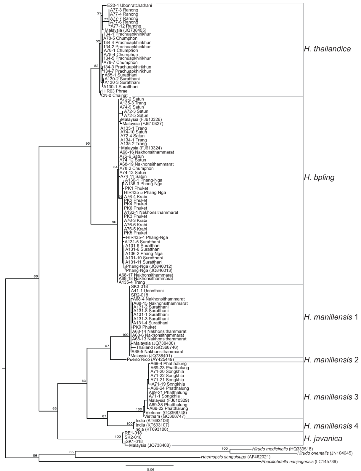
Fig. S1. ML tree generated by IQTREE
