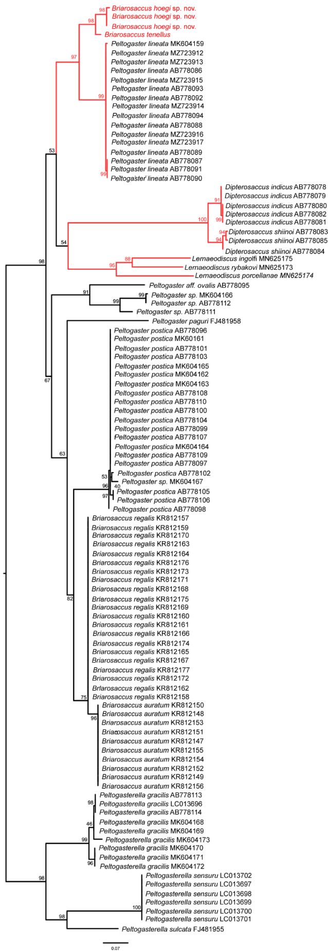
Fig. S4. Maximum likelihood tree of the family Peltogastridae for 16S gene fragments. Number above or under the brunches are bootstrap values. Red color highlighted differences between BI and ML phylogenetic reconstruction.
