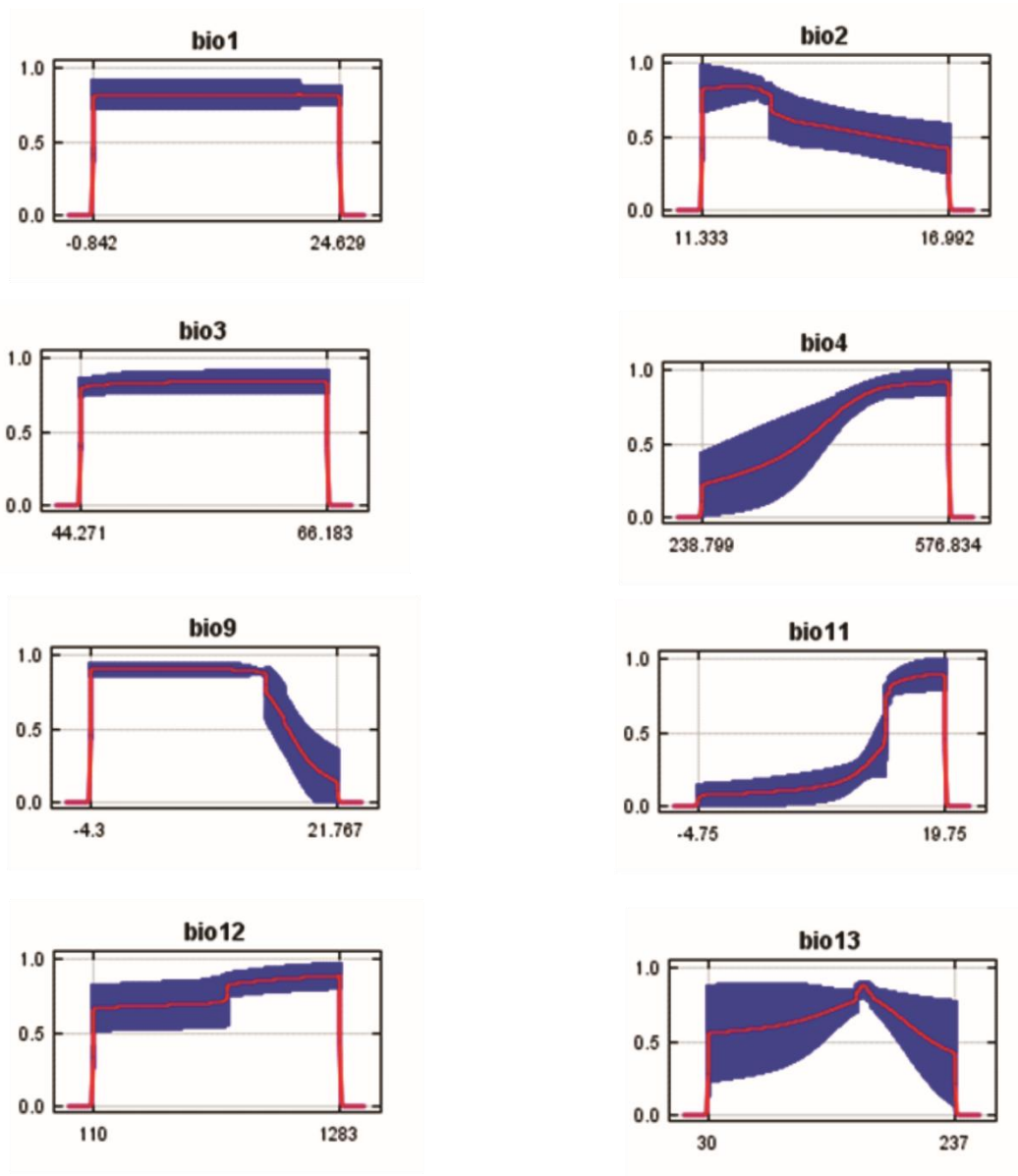
Fig. S3. P. argentina . Response curves.
