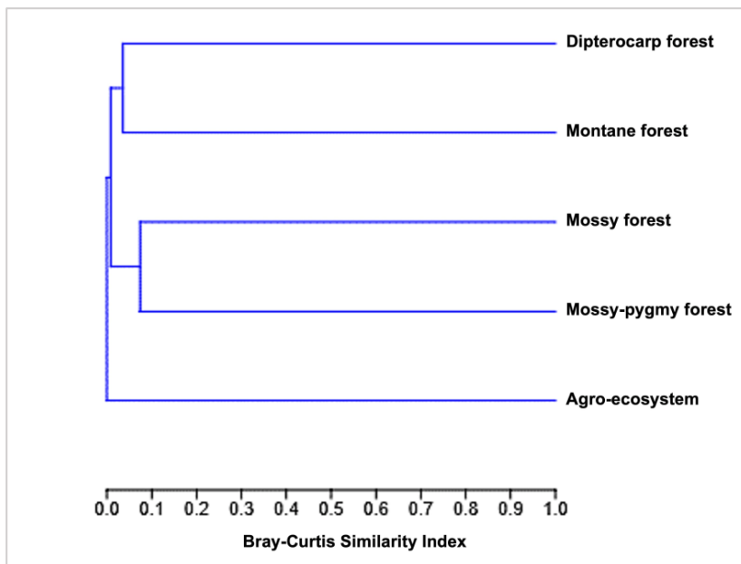
Fig. 7. Clustering analysis of all sample sites based on the Bray-Curtis similarity index.
