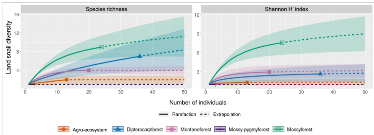
Fig. 6. Diversity accumulation curves of land snails across five survey sites in Mt. Hamiguitan, generated using iNEXT with 95% confidence intervals. The curves represent Hill numbers for species richness ( q = 0 ) and Shannon diversity ( q = 1 ), illustrating diversity patterns among the sites.
