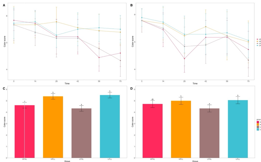
Fig. 5. Time course and endpoint of color score across treatments. The variety of color scores of S. pistillata ( n = 72 ) and P. damicornis ( n = 72 ). The variety of color scores in 70 days of S. pistillata (A) and P. damicornis , (B) measured every 14 days. Last measurement of color score of S. pistillata (C) and P. damicornis (D). Points/bars show mean \pm SE ( n = 18 fragments per group). Different letters indicate significant pairwise differences at p < 0.05 .
