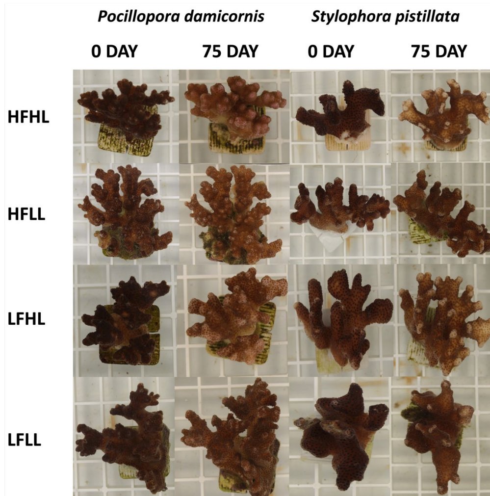
Fig 2. Photos of S. pistillata and P. damicornis branches under the different treatments at 0 days and 75 days. HFHL, high feeding regimes with high light; HFLL, high feeding regimes with low light; LFHL, low feeding regimes with high light; LFLL, low feeding regimes with low light.
