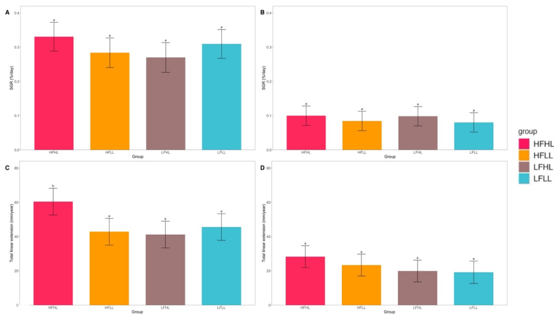
Fig. 4. Specific growth rate and total annual linear growth across treatments. Specific growth rate (% day -1 ; A–B) and total annual linear growth rate (mm yr -1 ; C–D) for S. pistillata (A, C; n = 72 ) and P. damicornis (B, D; n = 72 ) under HFHL, HFLL, LFHL, and LFLL. Bars show mean \pm SE ( n = 18 fragments per group). Different letters indicate significant pairwise differences at p < 0.05 .
